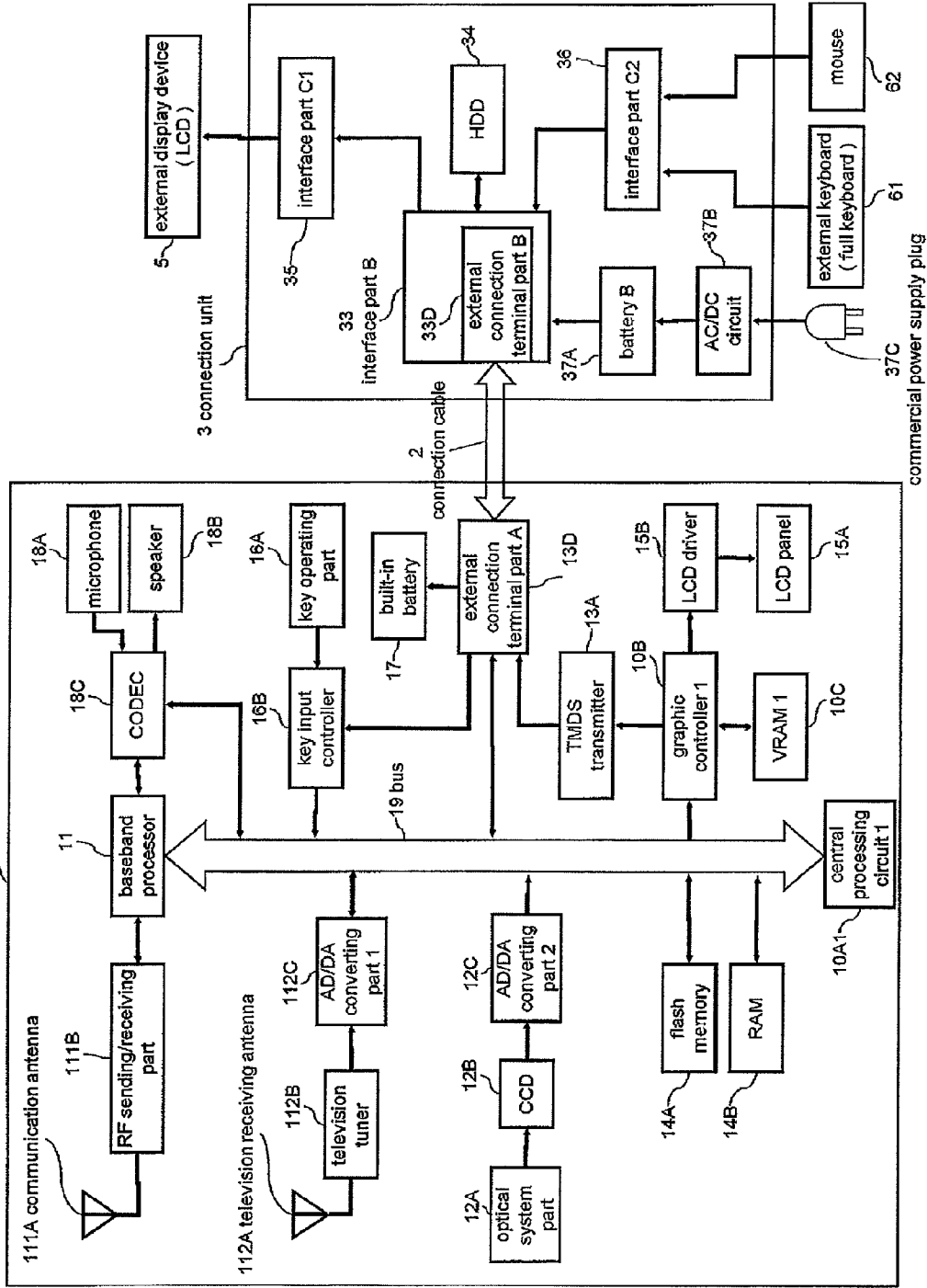
[FIG. 1] 1 mobile telephone unit
